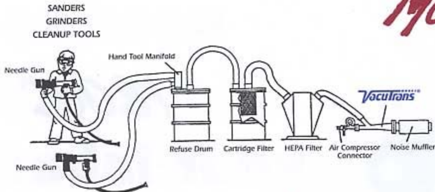
Example Hazardous Materials Package
