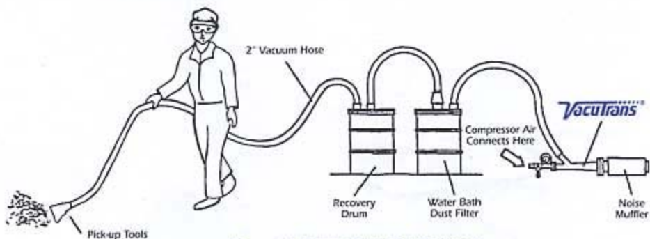
Example Drum Transfer Package
