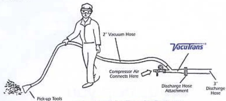
Example Direct Transfer Package
